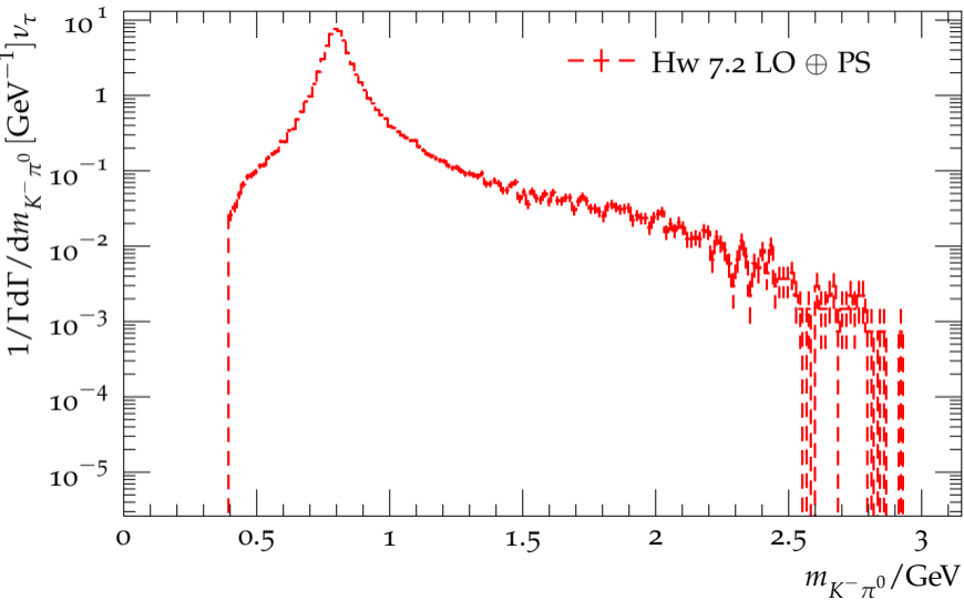
Mass distribution of the hadrons for \tau^- \rightarrow K^- \pi^0
