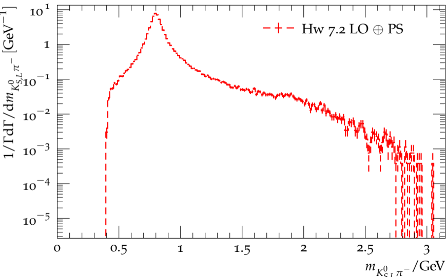
Mass distribution of the hadrons for \tau^- \rightarrow K_{S,L}^0 \pi^- \nu_\tau
