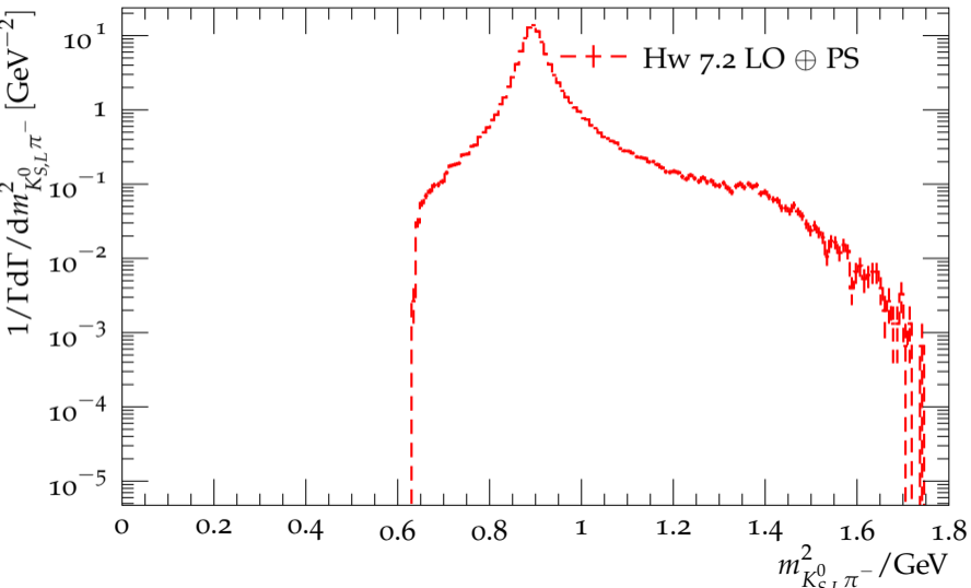
Mass distribution of the hadrons for \tau^- \rightarrow K_{S,L}^0 \pi^- \nu_\tau
