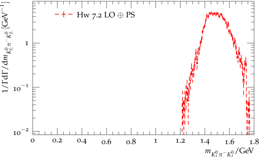
Distribution of the hadronic mass in \tau^- \rightarrow K_L^0 \pi^- K_L^0 \nu_\tau
