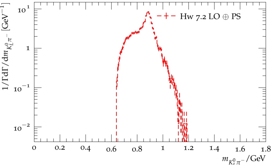
Distribution of the K_L^0\pi^- mass in \tau^- \rightarrow K_L^0\pi^- K_L^0\nu_\tau
