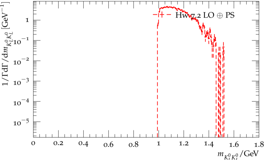
Distribution of the K_L^0 K_L^0 mass in \tau^- \rightarrow K_L^0 \pi^- K_L^0 \nu_\tau
