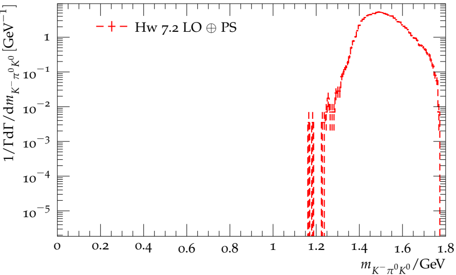
Distribution of the hadronic mass in \tau^- \rightarrow K^- \pi^0 K^0 \nu_\tau
