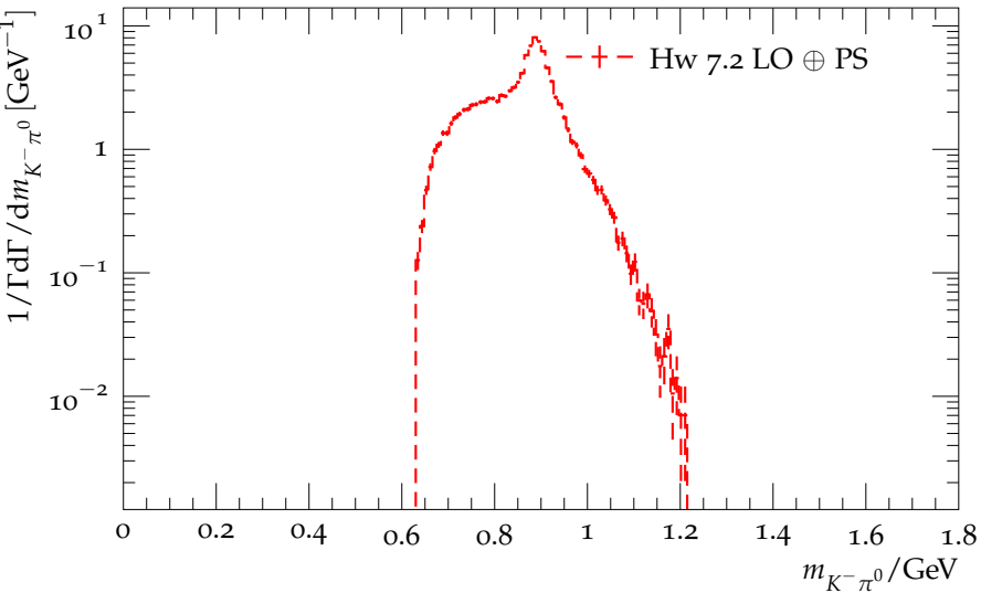
Distribution of the K^- \pi^0 mass in \tau^- \rightarrow K^- \pi^0 K^0 \nu_\tau
