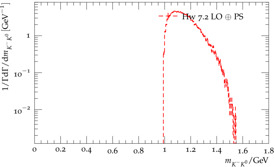
Distribution of the K^- K^0 mass in \tau^- \rightarrow K^- \pi^0 K^0 \nu_\tau
