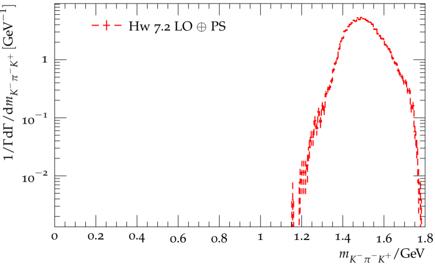
Distribution of the hadronic mass in \tau^- \rightarrow K^- \pi^- K^+ \nu_\tau
