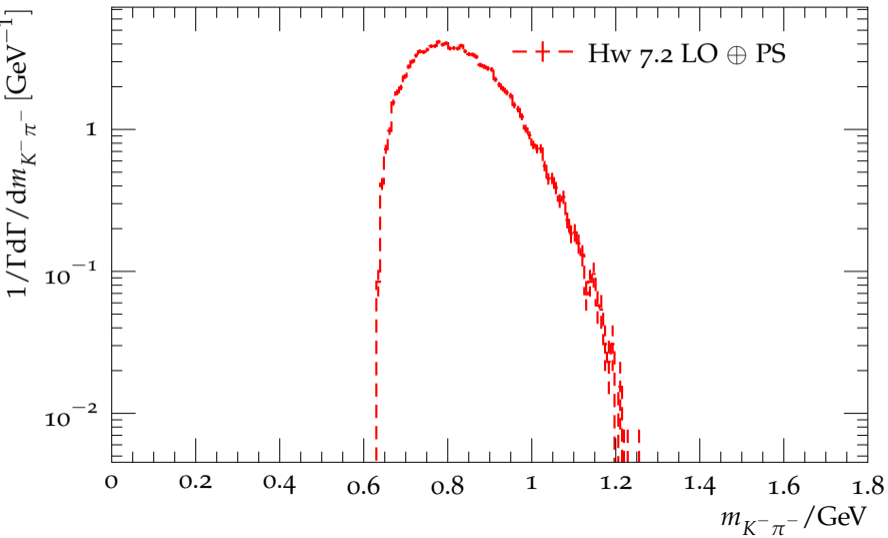
Distribution of the K^- \pi^- mass in \tau^- \rightarrow K^- \pi^- K^+ \nu_\tau
