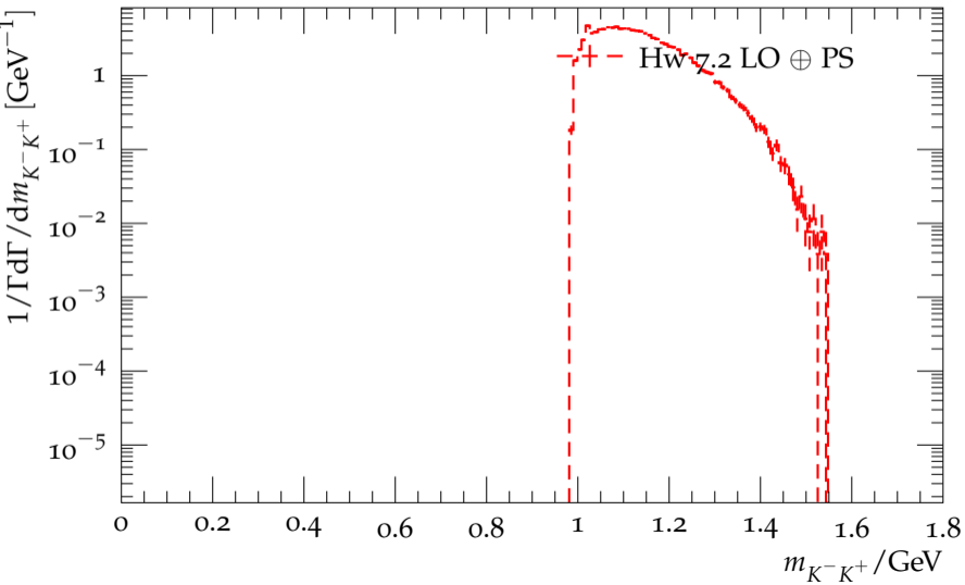
Distribution of the K^-K^+ mass in \tau^- \rightarrow K^- \pi^- K^+ \nu_\tau
