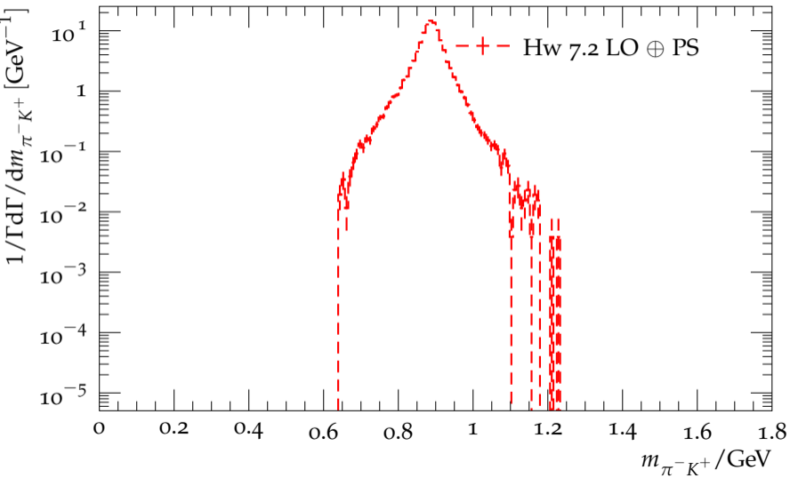
Distribution of the \pi^- K^+ mass in \tau^- \rightarrow K^- \pi^- K^+ \nu_\tau
