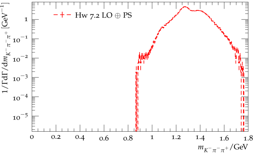
Distribution of the hadronic mass in \tau^- \rightarrow K^- \pi^- \pi^+ \nu_\tau
