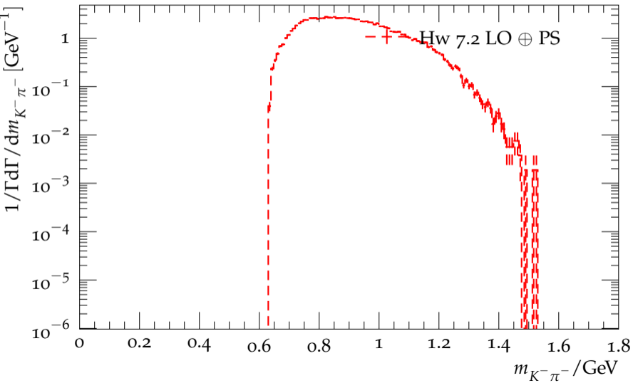
Distribution of the K^- \pi^- mass in \tau^- \rightarrow K^- \pi^- \pi^+ \nu_\tau
