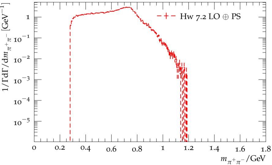
Distribution of the \pi^+\pi^- mass in \tau^- \rightarrow K^-\pi^-\pi^+\nu_\tau
