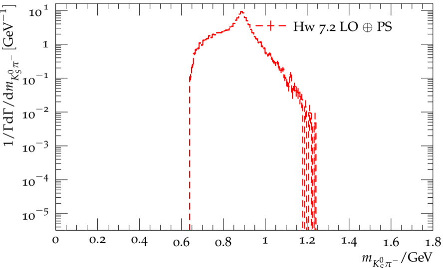
Distribution of the K_S^0\pi^- mass in \tau^- \rightarrow K_S^0\pi^- K_L^0\nu_\tau
