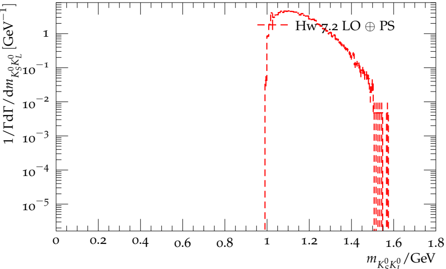
Distribution of the K_S^0 K_L^0 mass in \tau^- \rightarrow K_S^0 \pi^- K_L^0 \nu_\tau
