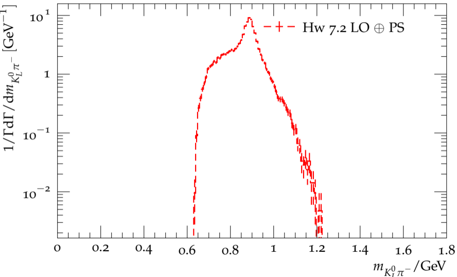
Distribution of the K_L^0\pi^- mass in \tau^- \rightarrow K_S^0\pi^- K_L^0\nu_\tau
