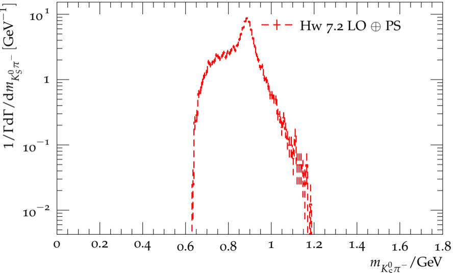
Distribution of the K_S^0\pi^- mass in \tau^- \rightarrow K_S^0\pi^- K_S^0\nu_\tau
