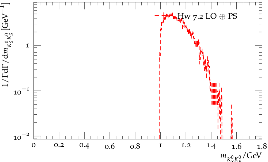
Distribution of the K_S^0 K_S^0 mass in \tau^- \rightarrow K_S^0 \pi^- K_S^0 \nu_\tau
