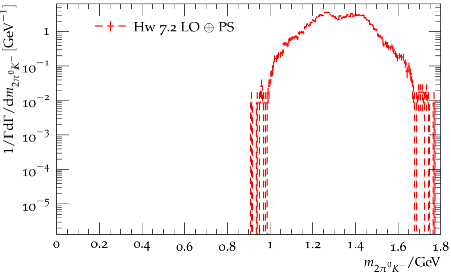
Distribution of the hadronic mass in \tau^- \rightarrow 2\pi^0 K^- \nu_\tau
