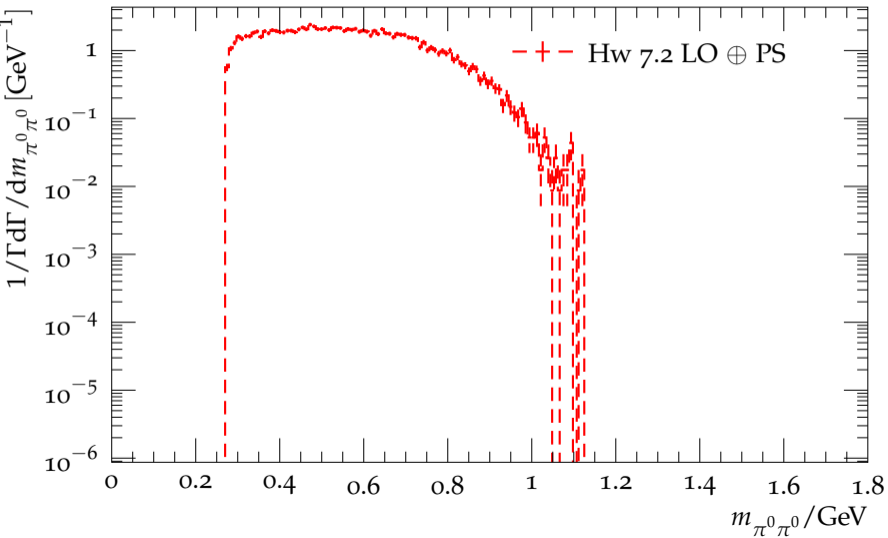
Distribution of the \pi^0\pi^0 mass in \tau^- \rightarrow 2\pi^0 K^- \nu_\tau
