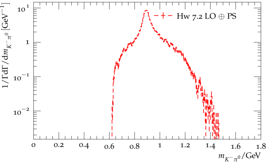
Distribution of the K^- \pi^0 mass in \tau^- \rightarrow 2\pi^0 K^- \nu_\tau
