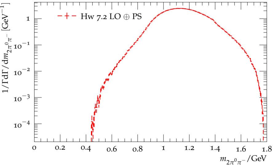
Distribution of the hadronic mass in \tau^- \rightarrow 2\pi^0\pi^- \nu_\tau
