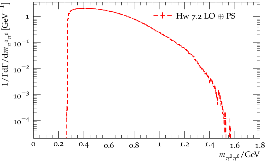
Distribution of the \pi^0\pi^0 mass in \tau^- \rightarrow 2\pi^0\pi^-\nu_\tau
