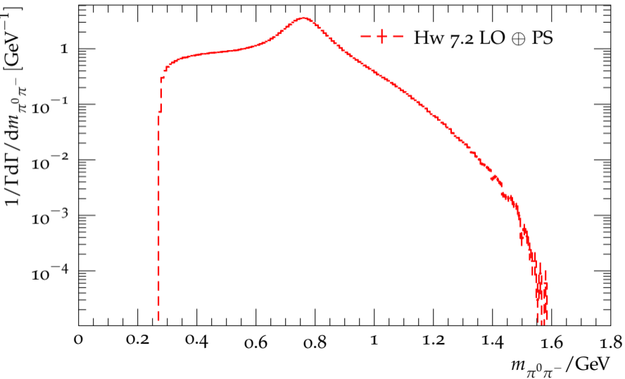
Distribution of the \pi^0\pi^- mass in \tau^- \rightarrow 2\pi^0\pi^- \nu_\tau
