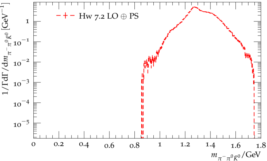
Distribution of the hadronic mass in \tau^- \rightarrow \pi^- \pi^0 \bar{K}^0 \nu_\tau
