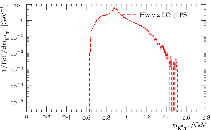
Distribution of the \bar{K}^0 \pi^- mass in \tau^- \rightarrow \pi^- \pi^0 \bar{K}^0 \nu_\tau
