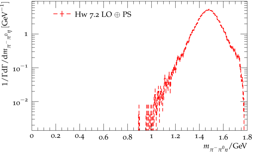
Distribution of the hadronic mass in \tau^- \rightarrow \pi^- \pi^0 \eta \nu_\tau
