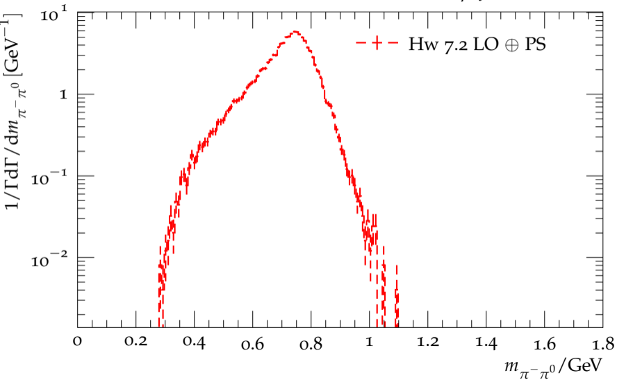
Distribution of the \pi^- \pi^0 mass in \tau^- \rightarrow \pi^- \pi^0 \eta \nu_\tau
