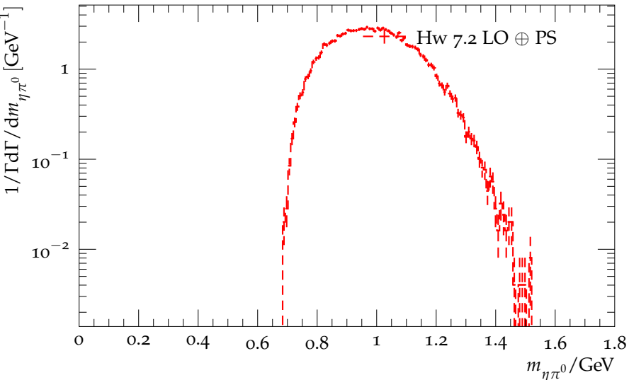
Distribution of the \eta\pi^0 mass in \tau^- \rightarrow \pi^- \pi^0 \eta \nu_\tau
