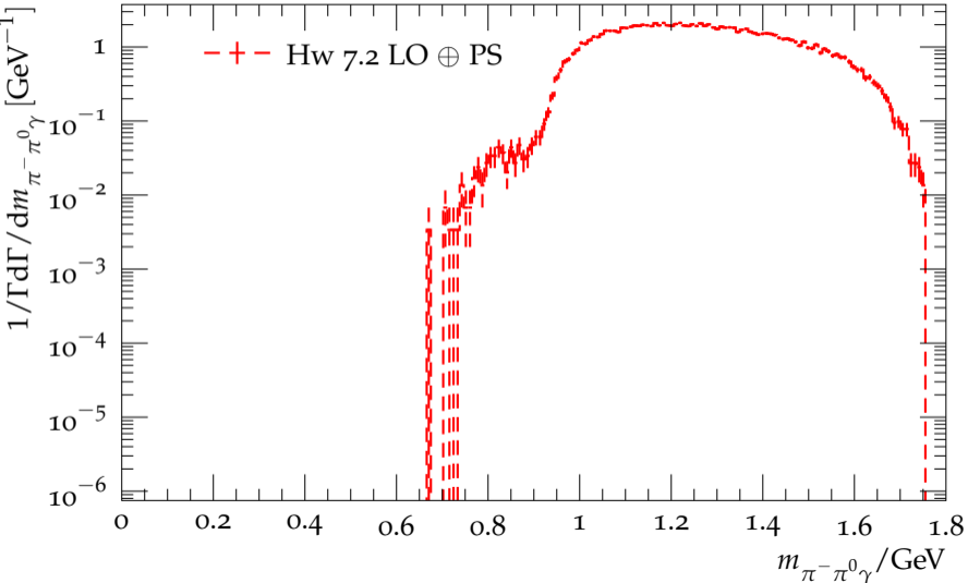
Distribution of the hadronic mass in \tau^- \rightarrow \pi^- \pi^0 \gamma \nu_\tau
