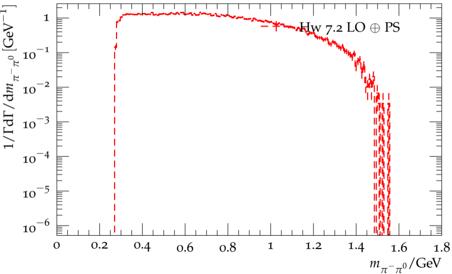
Distribution of the \pi^- \pi^0 mass in \tau^- \rightarrow \pi^- \pi^0 \gamma \nu_\tau
