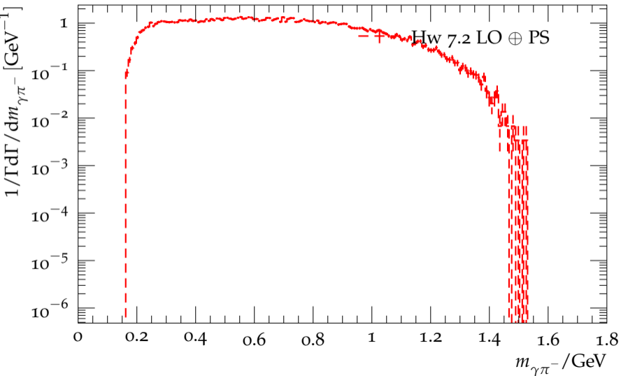
Distribution of the \gamma\pi^- mass in \tau^- \rightarrow \pi^- \pi^0 \gamma \nu_\tau
