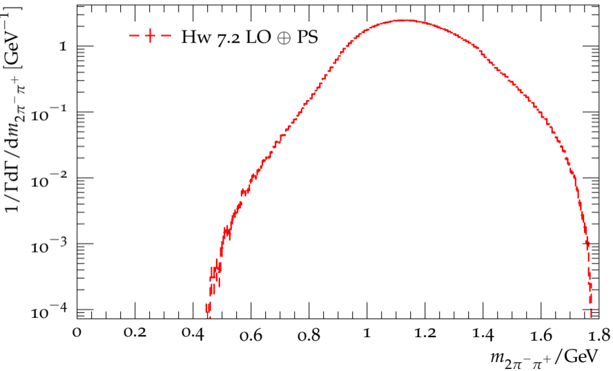
Distribution of the hadronic mass in \tau^- \rightarrow 2\pi^- \pi^+ \nu_\tau
