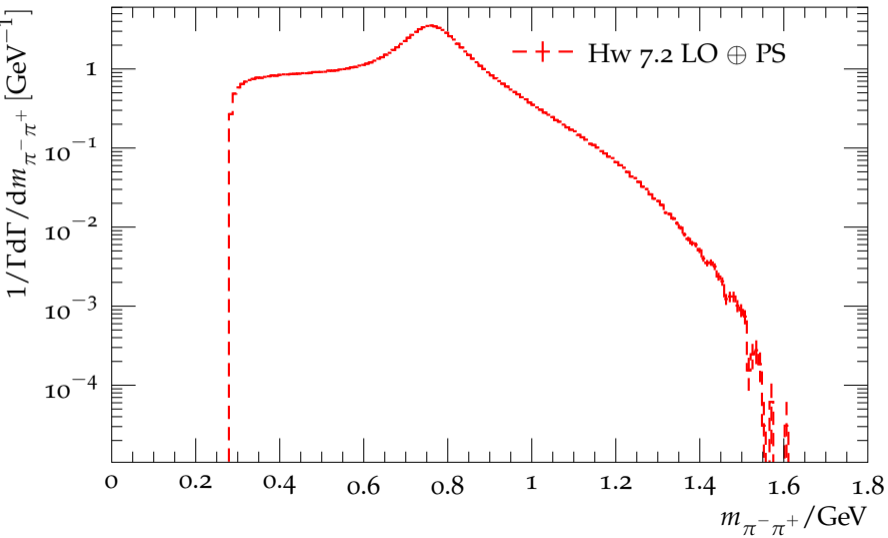
Distribution of the \pi^- \pi^+ mass in \tau^- \rightarrow 2\pi^- \pi^+ \nu_\tau
