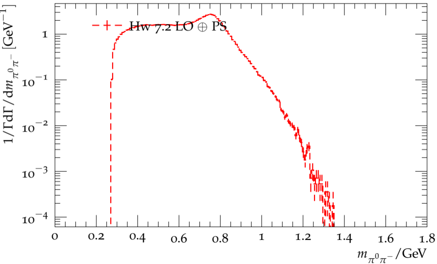
Distribution of the \pi^0\pi^- mass in \tau^- \rightarrow 3\pi^0\pi^- \nu_\tau
