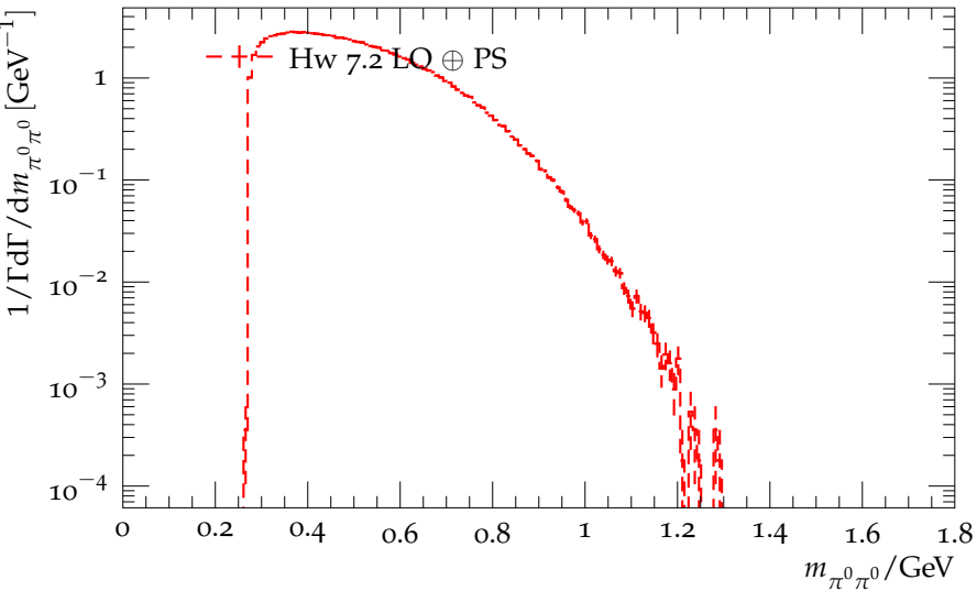
Distribution of the \pi^0\pi^0 mass in \tau^- \rightarrow 3\pi^0\pi^-\nu_\tau
