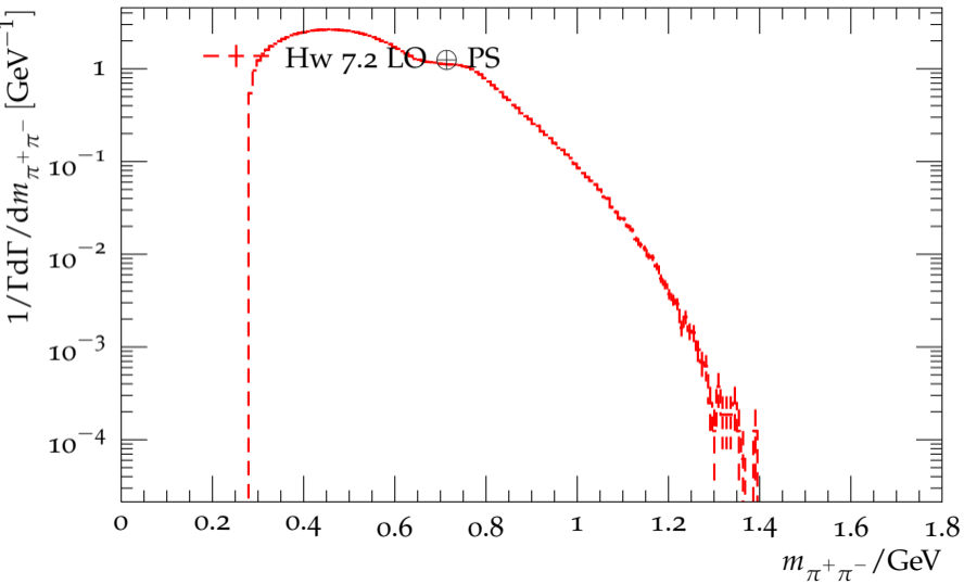
Distribution of the \pi^+\pi^- mass in \tau^- \rightarrow \pi^0\pi^+2\pi^-\nu_\tau
