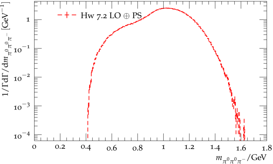
Distribution of the \pi^0\pi^0\pi^- mass in \tau^- \rightarrow 3\pi^0\pi^-\nu_\tau
