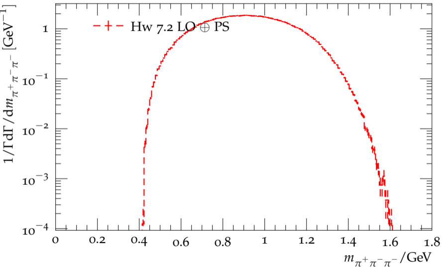
Distribution of the \pi^+\pi^-\pi^- mass in \tau^- \rightarrow \pi^0\pi^+2\pi^-\nu_\tau
