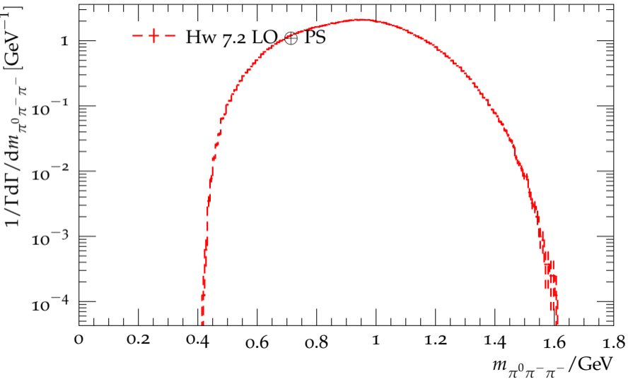
Distribution of the \pi^0 \pi^- \pi^- mass in \tau^- \rightarrow \pi^0 \pi^+ 2\pi^- \nu_\tau
