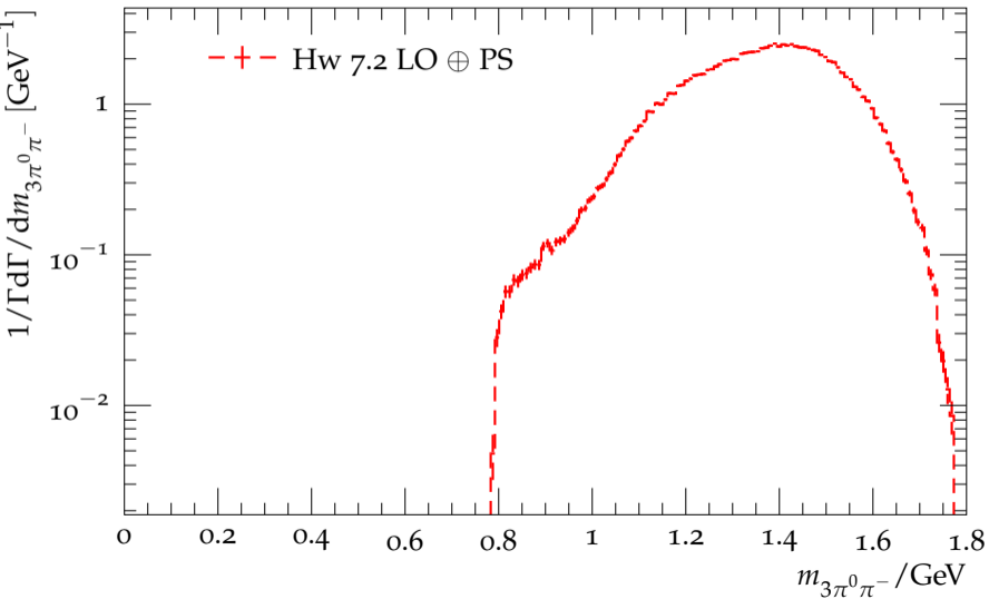
Distribution of the hadronic mass in \tau^- \rightarrow 3\pi^0 \pi^- \nu_\tau
