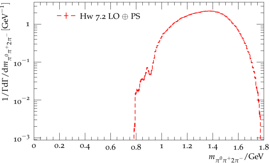
Distribution of the \pi^0\pi^+2\pi^- mass in \tau^- \rightarrow \pi^0\pi^+2\pi^-\nu_\tau
