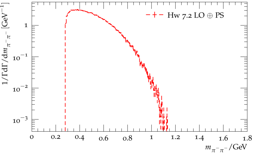
Distribution of the \pi^- \pi^- mass for \tau^- \rightarrow 2\pi^0 2\pi^- \pi^+ \nu_\tau
