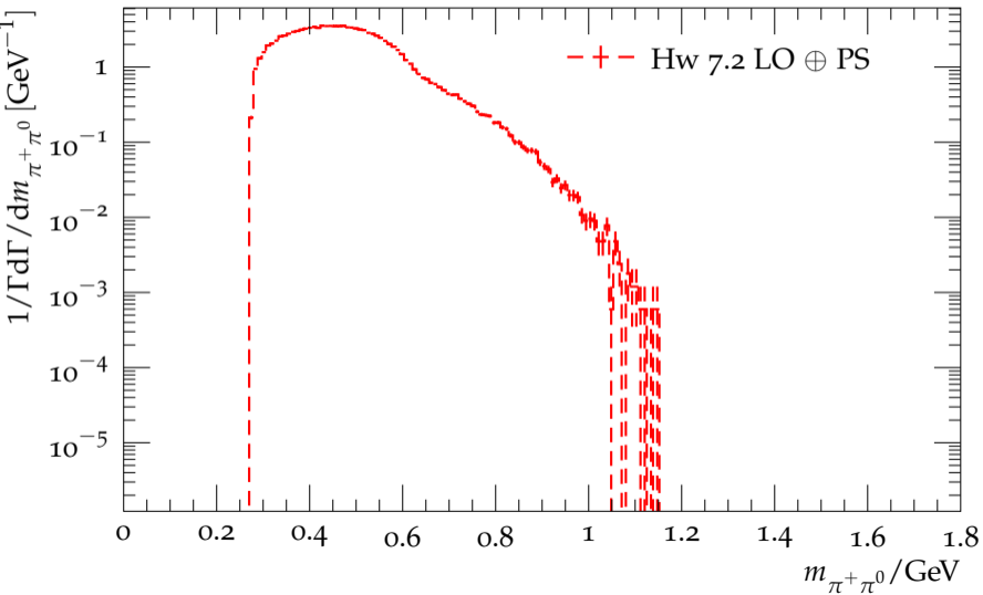
Distribution of the \pi^+\pi^0 mass for \tau^- \rightarrow 2\pi^0 2\pi^-\pi^+\nu_\tau
