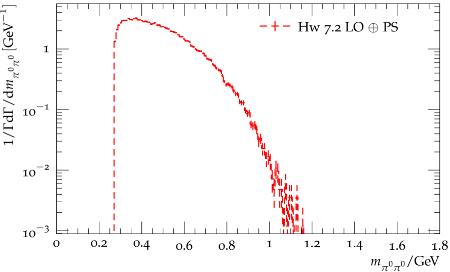
Distribution of the \pi^0\pi^0 mass for \tau^- \rightarrow 2\pi^0 2\pi^- \pi^+ \nu_\tau
