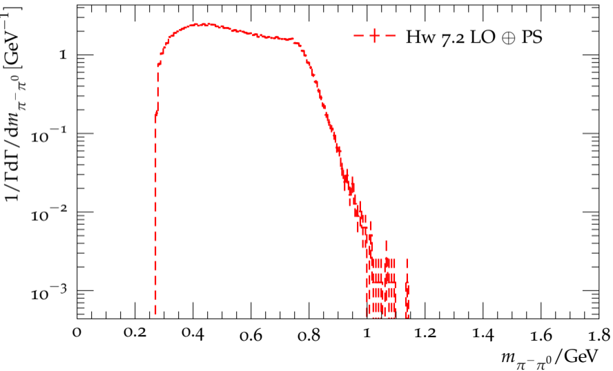
Distribution of the \pi^- \pi^0 mass for \tau^- \rightarrow 4\pi^0 \pi^- \nu_\tau
