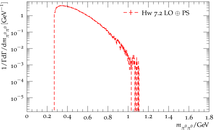
Distribution of the \pi^0\pi^0 mass for \tau^- \rightarrow 4\pi^0\pi^-\nu_\tau
